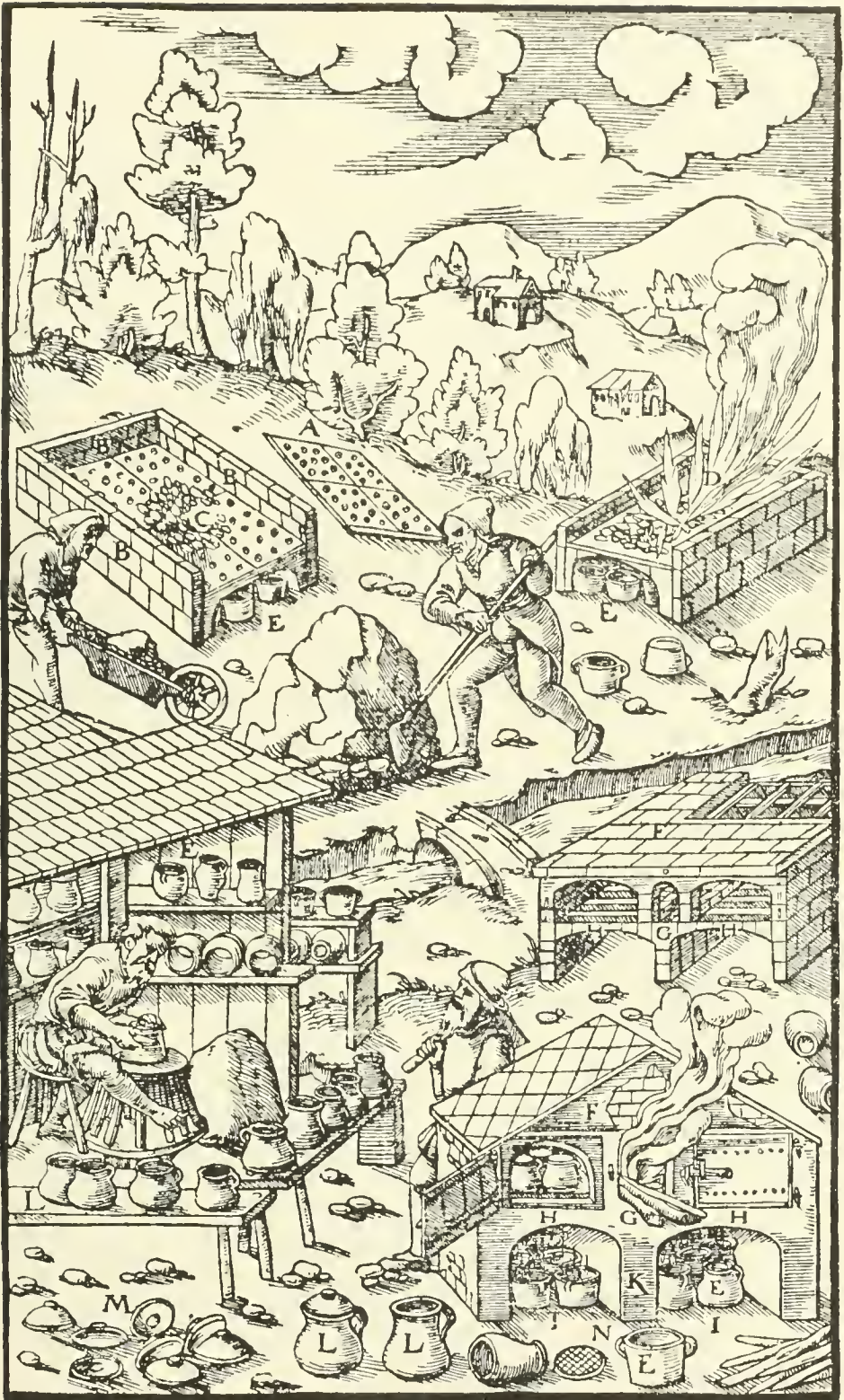
A—IRON PLATES FULL OF HOLES. B—WALLS. C—PLATE ON WHICH ORE IS PLACED. D—BURNING CHARCOAL PLACED ON THE ORE. E—POTS. F—FURNACE. G—MIDDLE PART OF UPPER CHAMBER. H—THE OTHER TWO COMPARTMENTS. I—DIVISIONS OF THE LOWER CHAMBER. K—MIDDLE WALL. L—POTS WHICH ARE FILLED WITH ORE. M—LIDS OF SAME POTS. N—GRATING.
